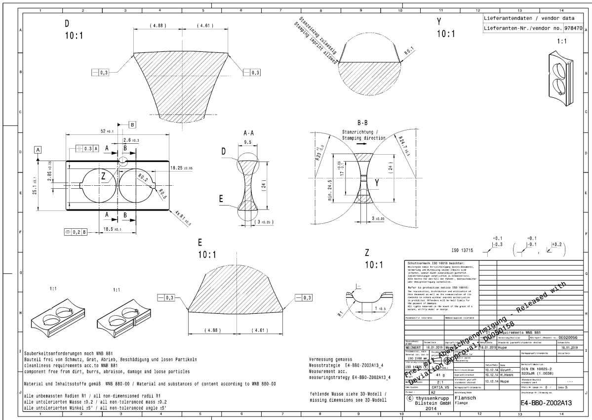
Figure 9: 10mm Flange
