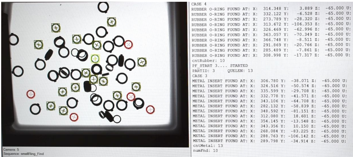
Figure 13: Epson Vision System
