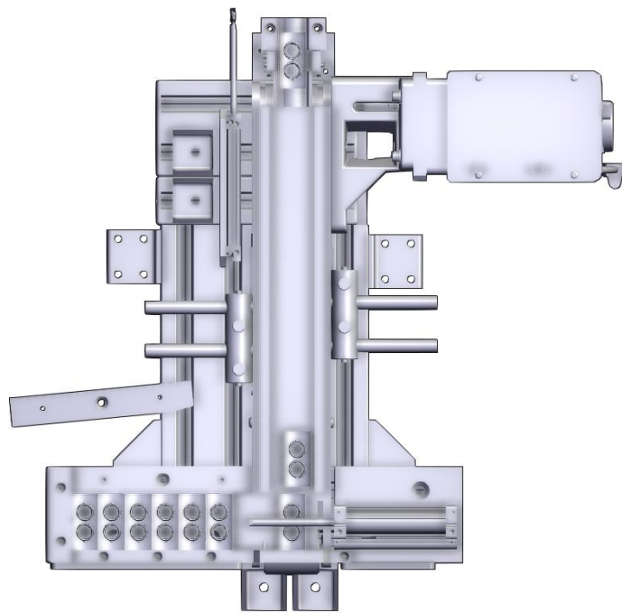
Figure 5: Flange Assembly Station
