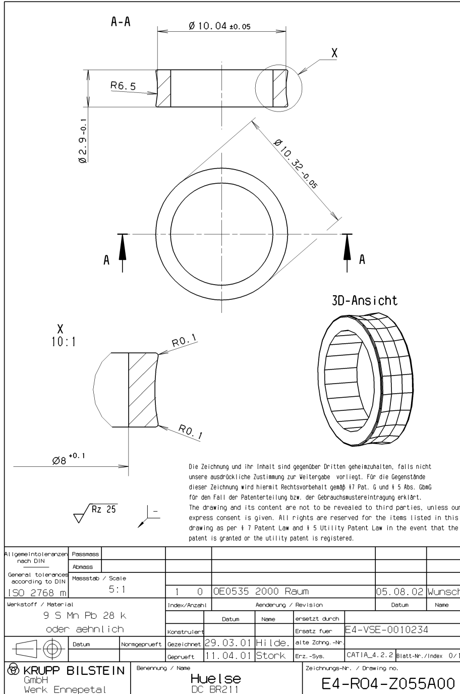
Figure 8: 8mm Metal Collar
