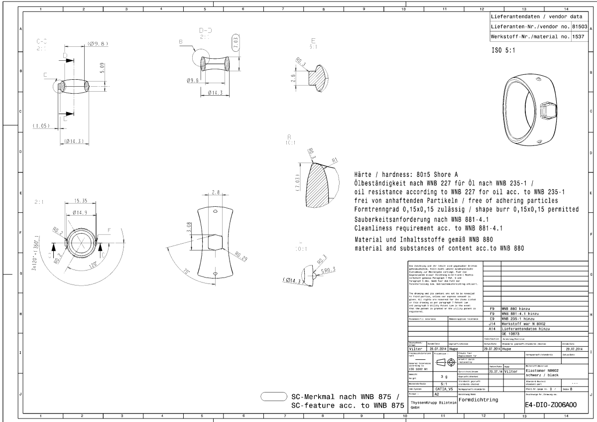
Figure 7: 8mm Rubber Sleeve
