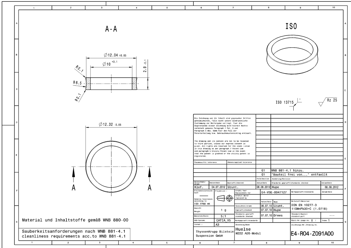
Figure 11: 10mm Metal Collar
