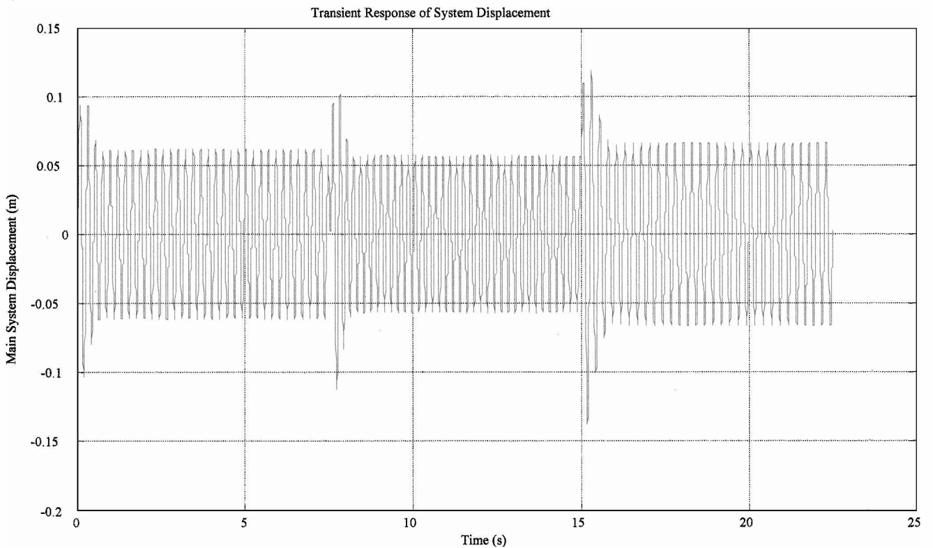
Fig. 6 Time response uncontrolled and AFCA.
