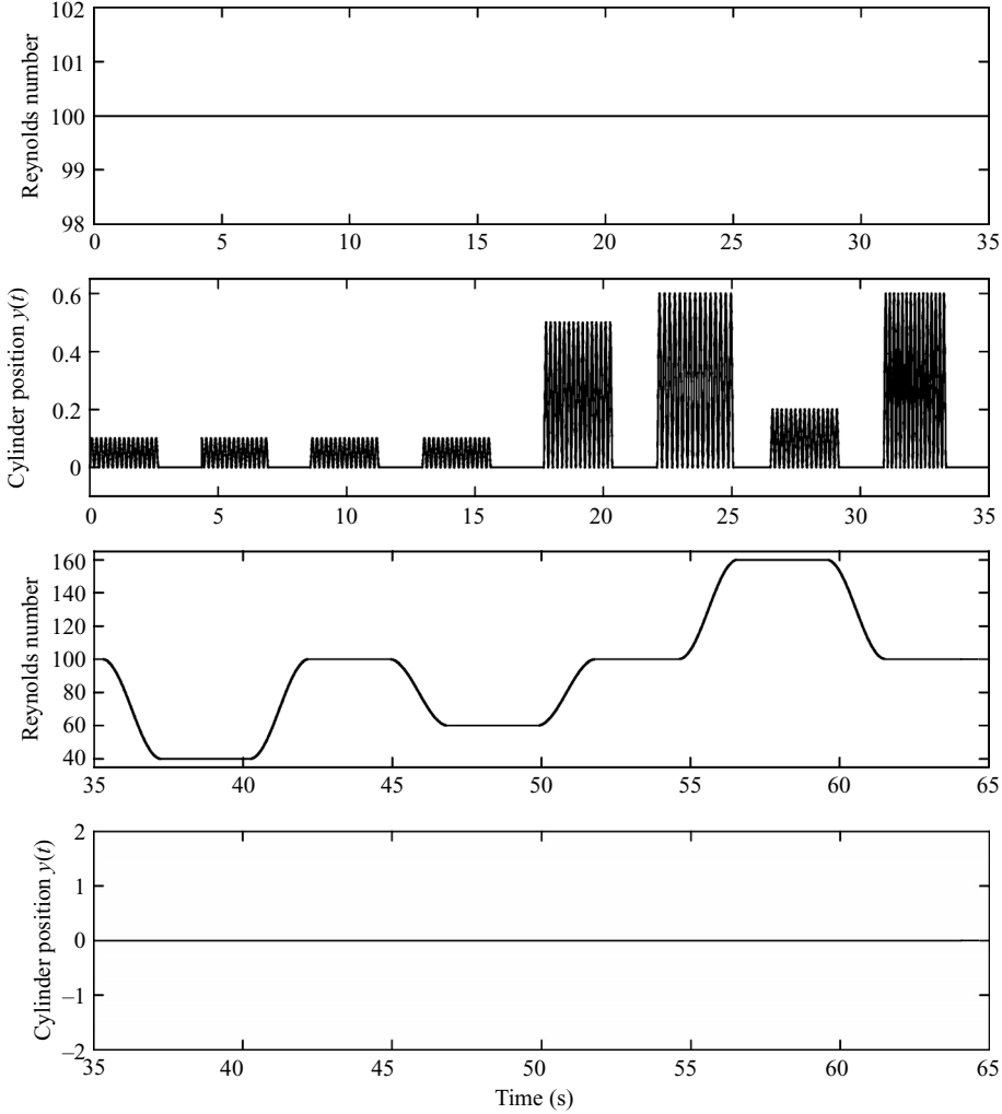
FIGURE 15. Neural network training data. t = 0 s to 35 s: cylinder displacement: Case 10 at 4 different phase angles of 0^\circ , 90^\circ , 180^\circ and 270^\circ , Case 1, Case 4, Case 5, Case 8 (see figure 8). t = 35 s to 64 s: Reynolds number transients: 100 \rightarrow 40 \rightarrow 100 \rightarrow 60 \rightarrow 100 \rightarrow 160 \rightarrow 100 .
