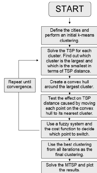
Fig. 7. Flowchart of fuzzy logic clustering used in genetic fuzzy clustering method [26]
