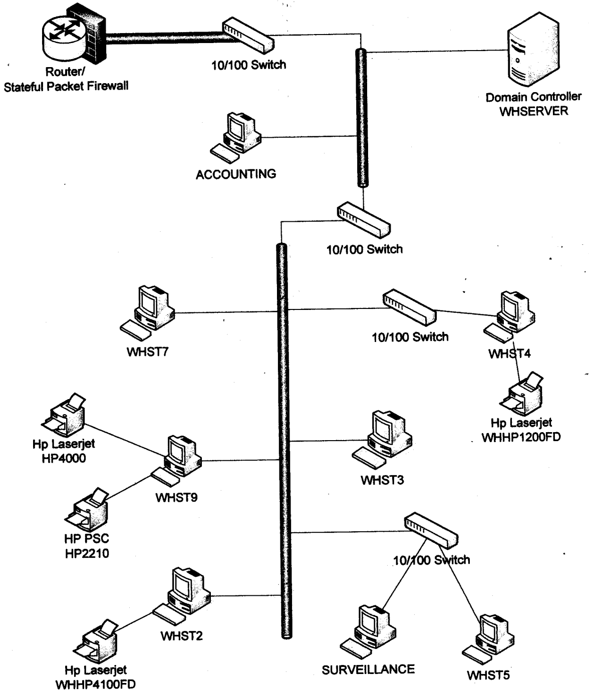
Figure 1: Western Hills LAN Design
