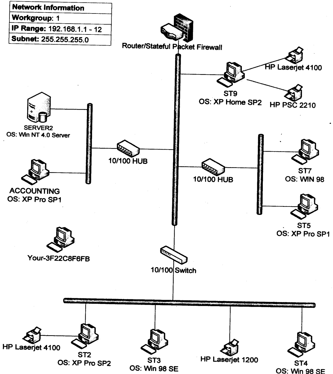
Figure 35: Western Hills LAN topology before upgrade
