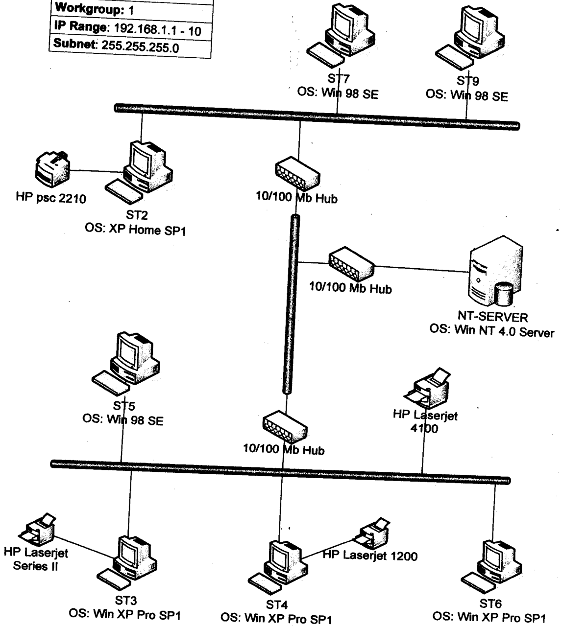
Figure 37: Montgomery LAN topology before upgrade
