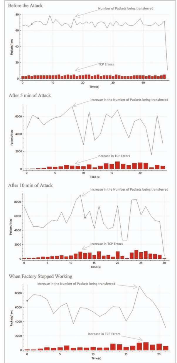
Fig. 3. Snapshots of packet transmission and TCP errors during DoS attack.
